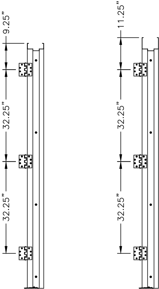
HINGE LOCATIONS 2" HEAD HINGE LOCATIONS 4" HEAD
