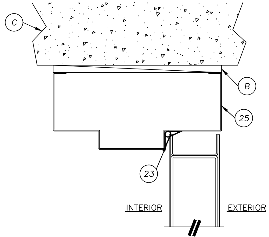
VERTICAL CROSS SECTION @ HEAD
